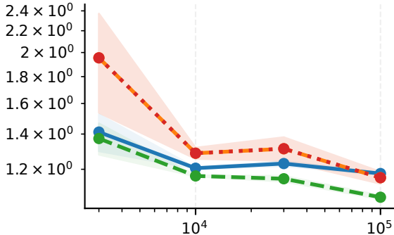
Oracle error vs n_{\text{train}} : Mean Integrated Absolute Error
